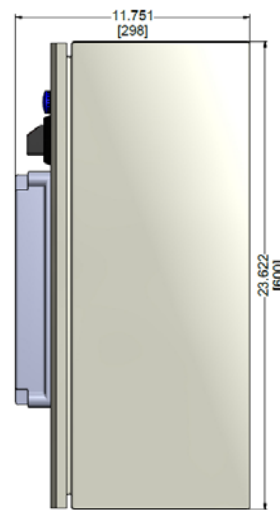
Side (NEMA 12 with cover)
